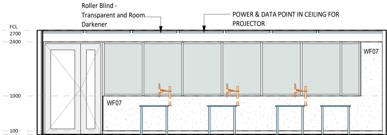
4 ELEVATION DETAIL 60-018 1 : 50
