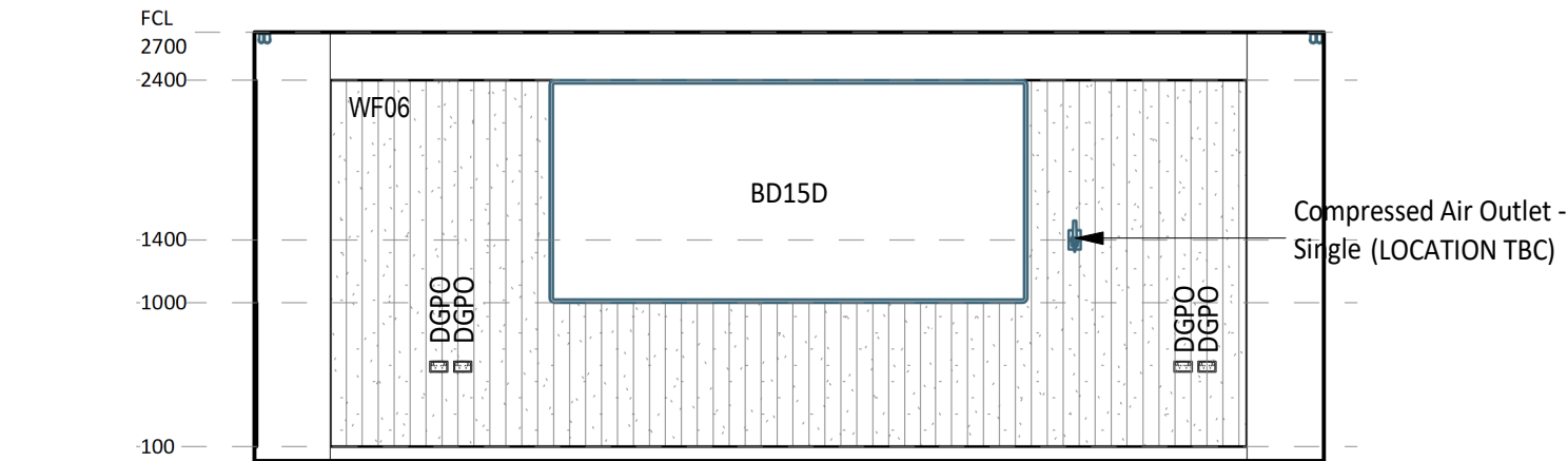
5 ELEVATION DETAIL 60-018 1 : 50
